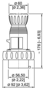
5-pole plug
