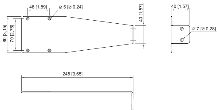
Mounting plate
