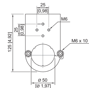
Mounting bracket for surfaces
