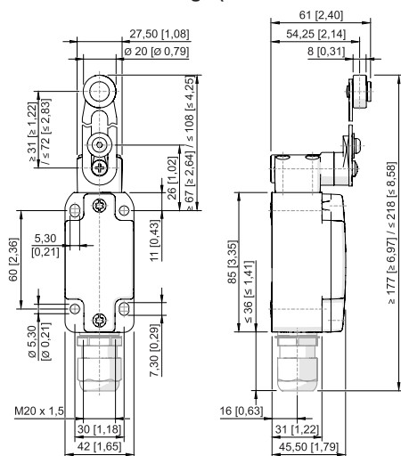
Swivelling lever 8070/2-5-DS-U60
