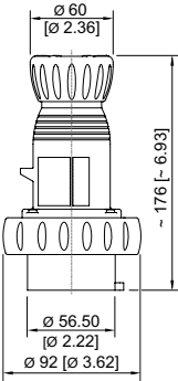
Plug 4 pole, 5 conductors
