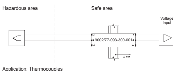
Application: Thermocouples
