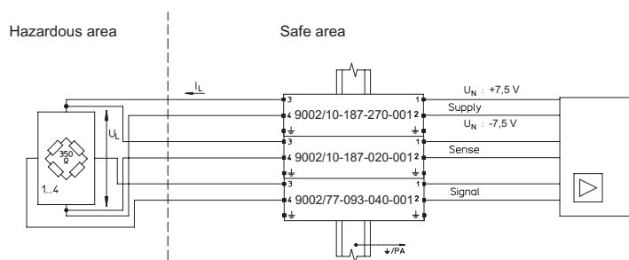
Application: Load cell (DMS) 350 Ω or 700 Ω 6-wire \pm 7.5 V (15 V) field circuit unearthed
