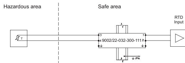
Application: Pt100, 2-wire circuit, field circuit unearthed
