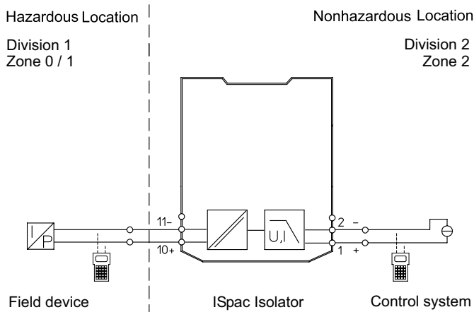
Connection diagram 9167/1
