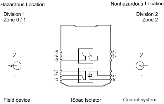
Connection Diagram 9172/21-11-00
