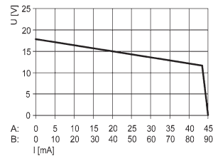
Output characteristic 9175/0-14-11, 9176/0-14-00
