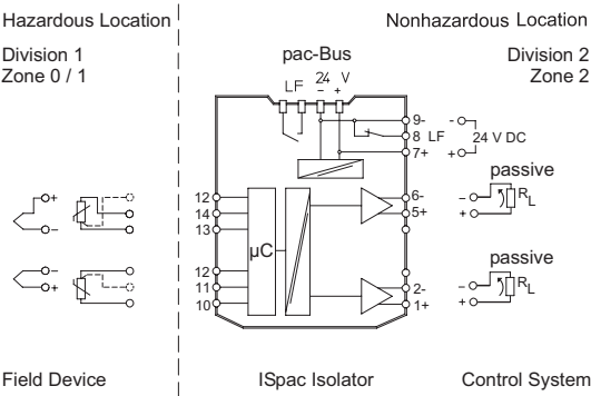
Connection diagram 9182/20-51-11
