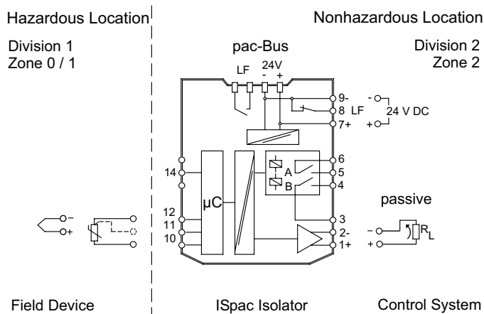
Connection diagram 9182/10-51-12; 9182/10-51-14
