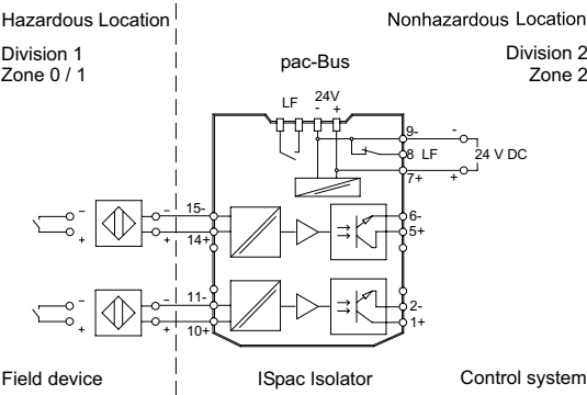
Connection diagram 9170/21-14-11
