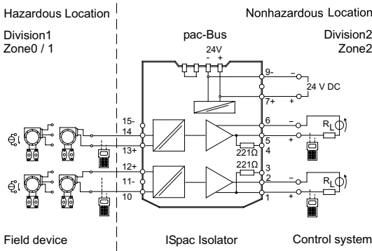
Connection diagram 9160/23-10-10
