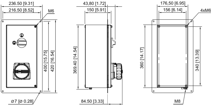
Dimensional Drawings (All Dimensions in mm [inches]) – Subject to Alterations
