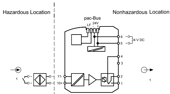
Connection diagram 9270/11-16-14
