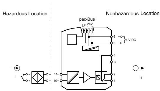
Connection diagram 9270/11-16-14
