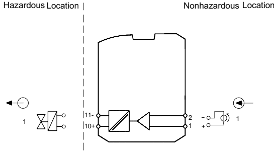
Connection diagram 9276/10
