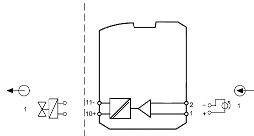
Connection diagram 9276/10
