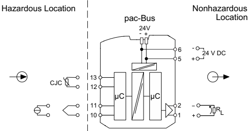
Connection diagram 9282/12-51-16
