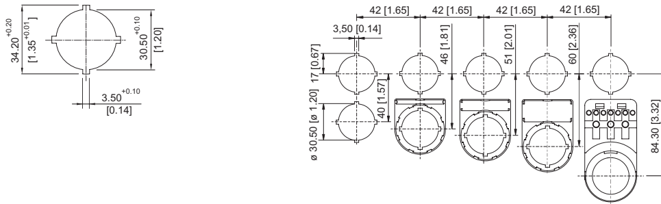
Cut-out with/without additional designation plate
