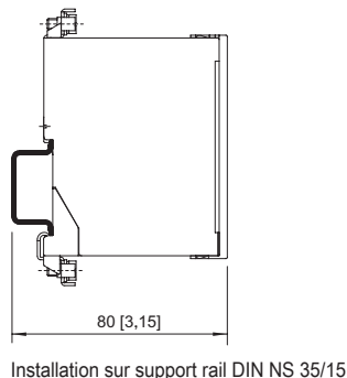
Installation sur support rail DIN NS 35/15
