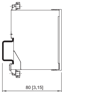
Installation sur support rail DIN NS 35/15
