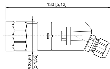
8003/...-001 Bouton-poussoir
