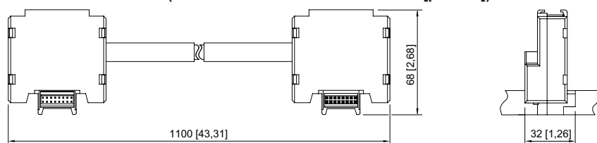
Rallonge BusRail
