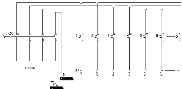
Diagrama unifilar 8146/5-ExV-...-.....1P-T
